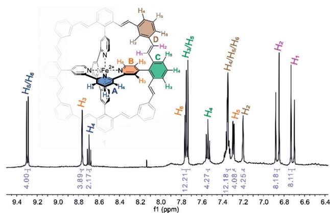
Figure 3. ^1\text{H} -NMR of the all- trans isomer of 1 with assignment of the signals.
